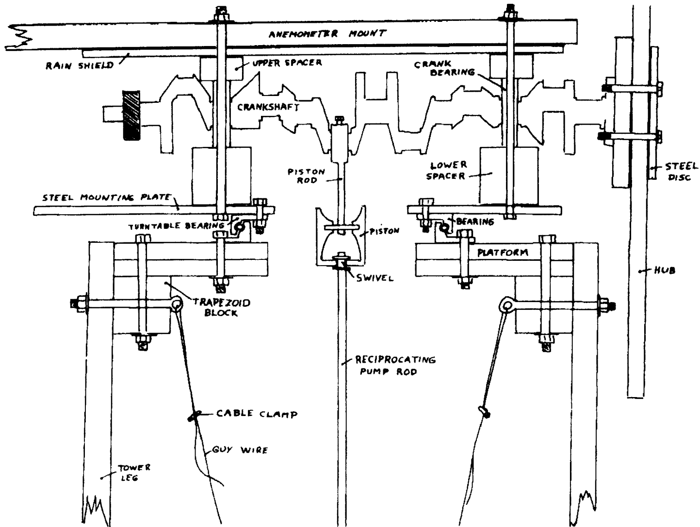
The turntable: an automobile crankshaft and piston are used to convert the rotating motion of the windmill rotor to the up-and-down motion of the pump rod.
